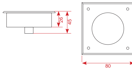
LedSpot 80 Square recessed diffused light "Kesseli"
