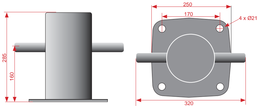
Led mooring bollard "Inari"
