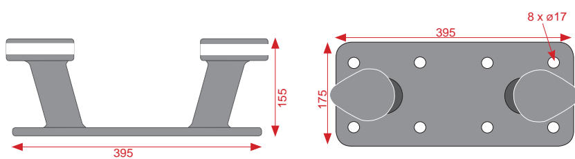
Led mooring bollard "Puula"
