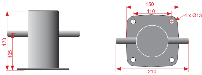
Led mooring bollard "Suvas"
