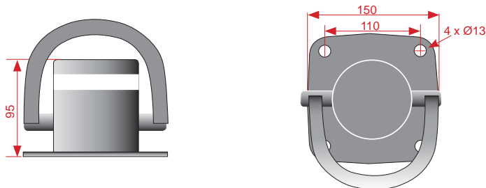
Led mooring bollard "Puro"
